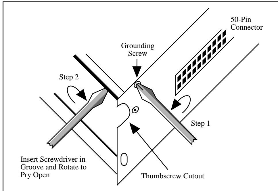
Figure 2-7. Cover Removal
